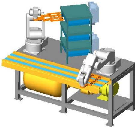
Kinematic Simulation of a Robotic Feed Arm for a QA Package Tester.
